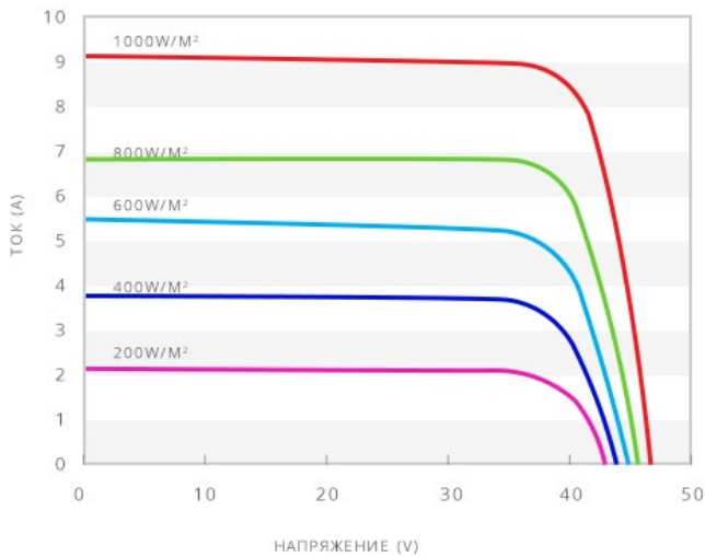
I-V Curves of PV module NEOSUN 320W at different light power
